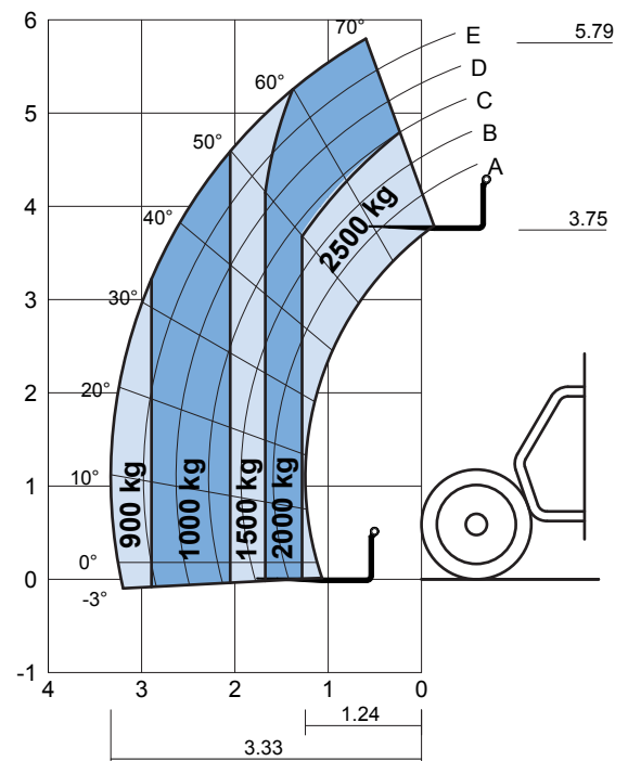
GTH-2506 AU.3 LOAD CHART WITH FORKS
